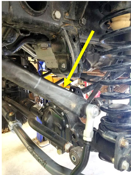
Figure 2. Sway Bar Disconnect and Pull Down
