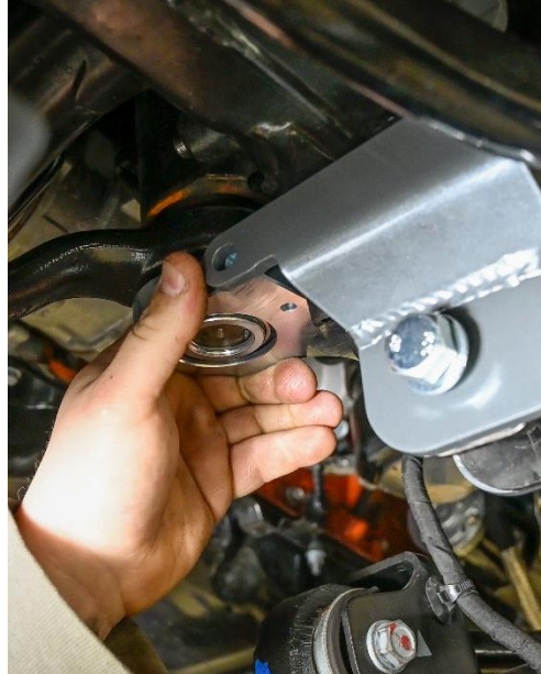
Figure 10. Installing Synergy Sealed Bearing Sector Shaft Brace
