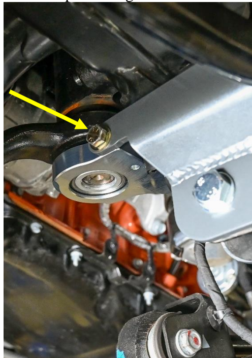
Figure 11. Installing Through Bolt in Synergy Sector Shaft Brace
